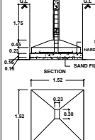
FOUNDATION DETAILS
