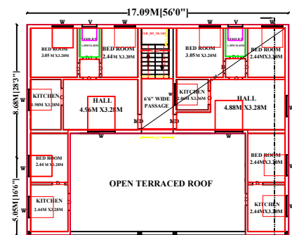
PROPOSED SECOND FLOOR - PLAN
