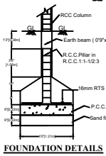
FOUNDATION DETAILS
