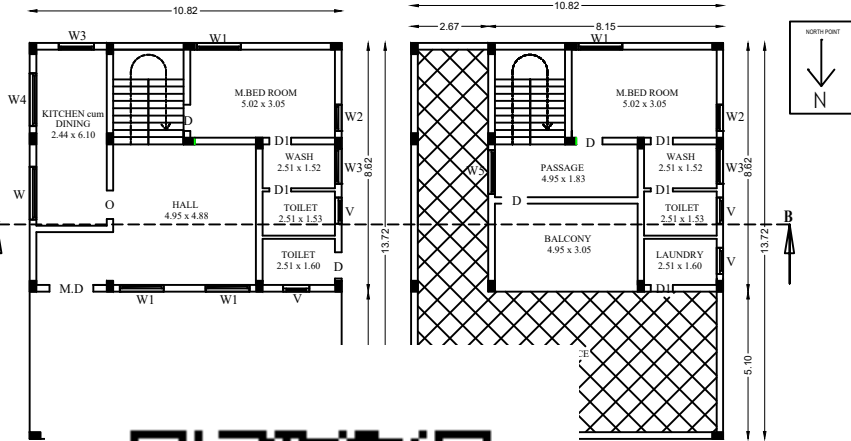
FLOOR PLAN
