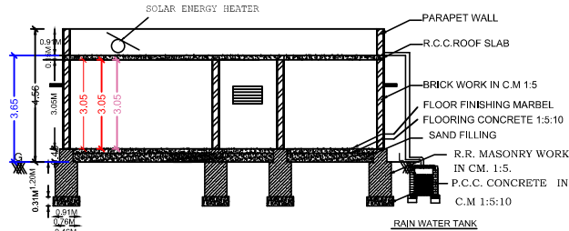
SECTION - XX
