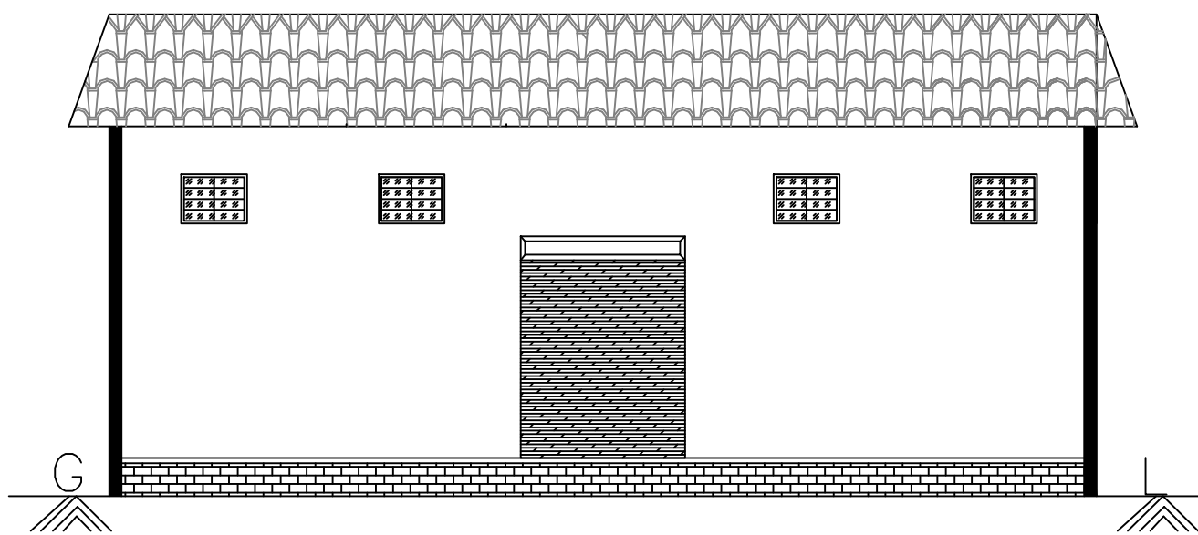
FRONT ELEVATION
