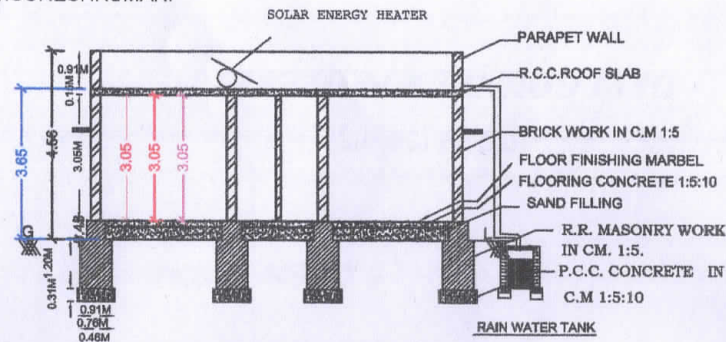
SECTION - XX
