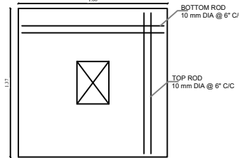
FOOTING PLAN
