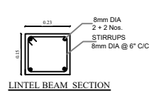
LINTEL BEAM SECTION
