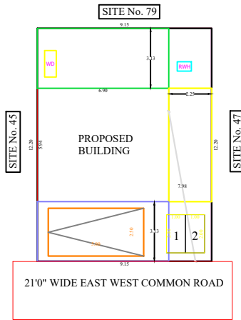
SITE PLAN
