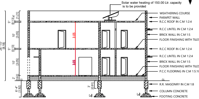
CROSS SECTION "AB"
