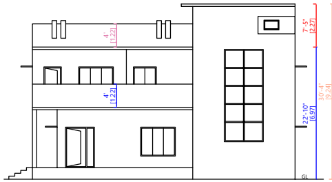
FRONT ELEVATION(NORTH SIDE VIEW)
