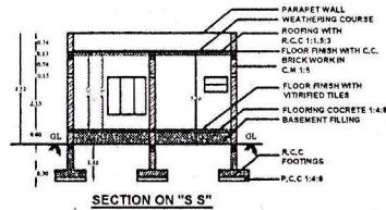
SECTION ON "S S"
