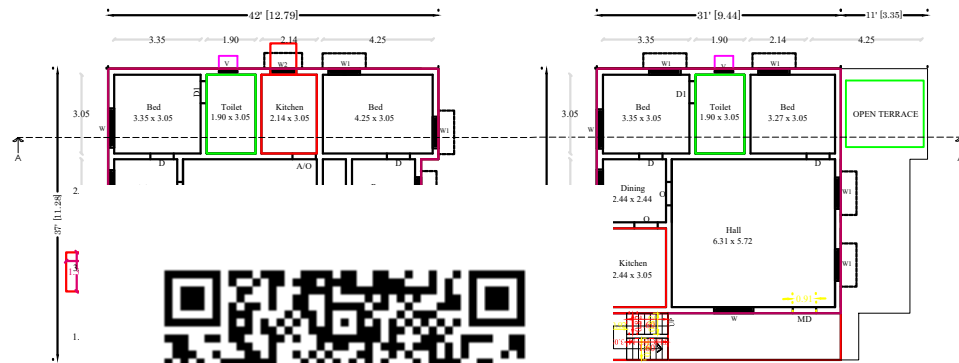
FIRST FLOOR PLAN SCALE:1:100 (PROPOSED BUILDING)
