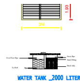
WATER TANK _2000 LITER
