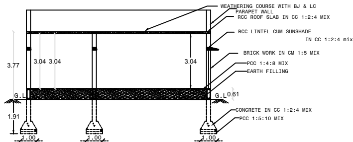
CROSS SECTION ON 'AA'
