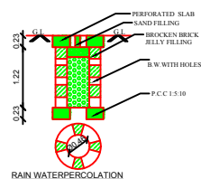
RAIN WATER PERCOLATION
