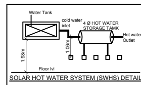
SOLAR HOT WATER SYSTEM (SWHS) DETAIL
