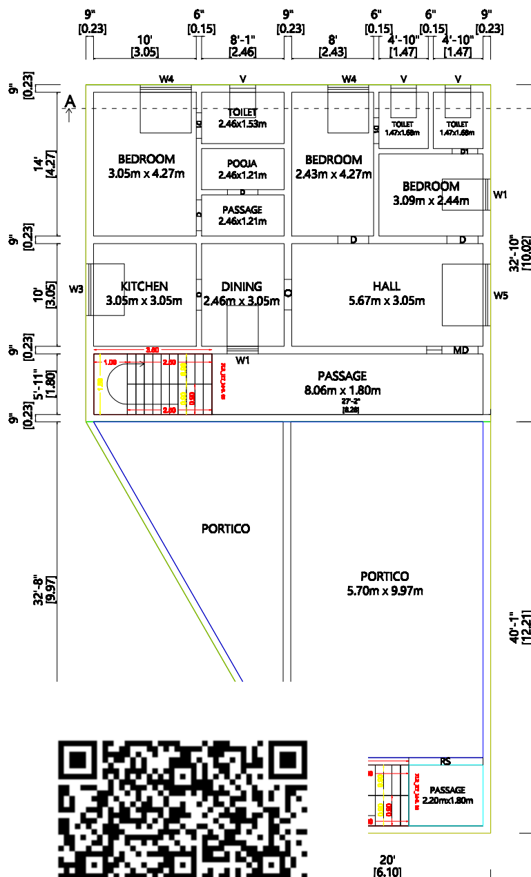
DDITIONAL PLAN
