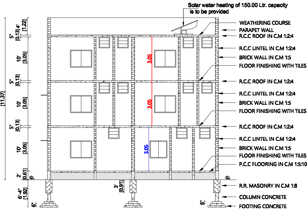
CROSS SECTION "AB"
