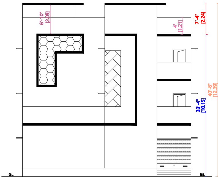
FRONT ELEVATION (EAST SIDE VIEW)
