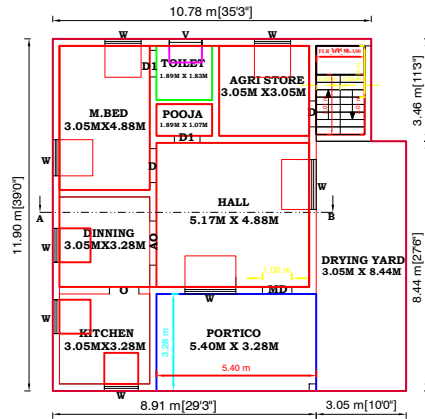
AGRI FARM HOUSE & DRYING YARD - PLAN
