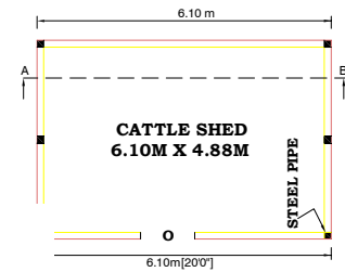
CATTLE SHED - PLAN
