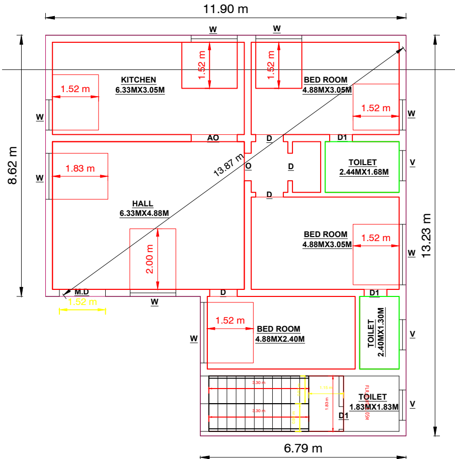
HOUSE PLAN
