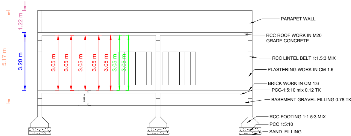
SECTION"AB"
