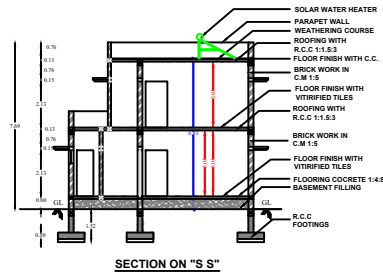
SECTION ON "S S"
