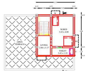
PROPOSED FIRST FLOOR PLAN
