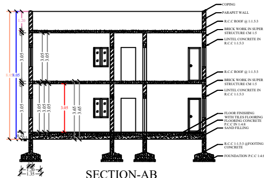
SECTION-AB
