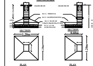
COLUMN FOOTING DETAILS
