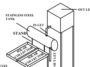
SOLAR HEATING WATER SYSTEM
