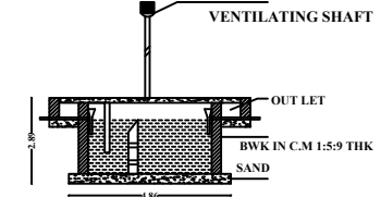
SECTION OF THE SEPTIC TANK
