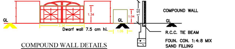
COMPOUND WALL DETAILS
