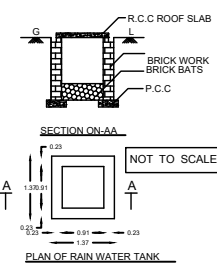
PLAN OF RAIN WATER TANK
