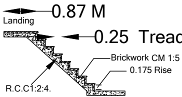
Staircase Details.
