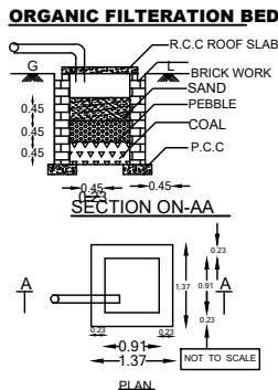
ORGANIC FILTRATION BED
