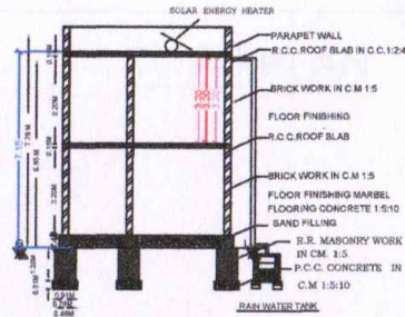
SECTION - XX
