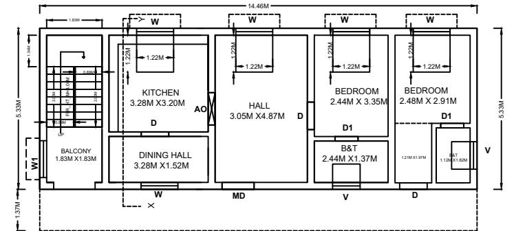
FIRST FLOOR PLAN SCALE : 1:100
