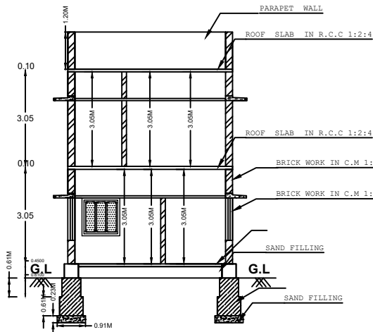
SECTION ON -XY.
