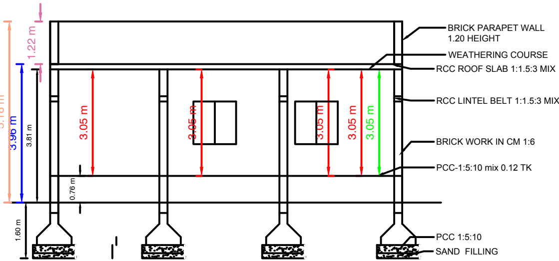
SECTION " AB "
