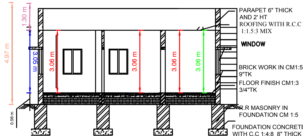
SECTIONAL VIEW A-A'
