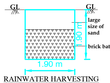
RAINWATER HARVESTING RWH TANK CAPACITY=2000LITER
