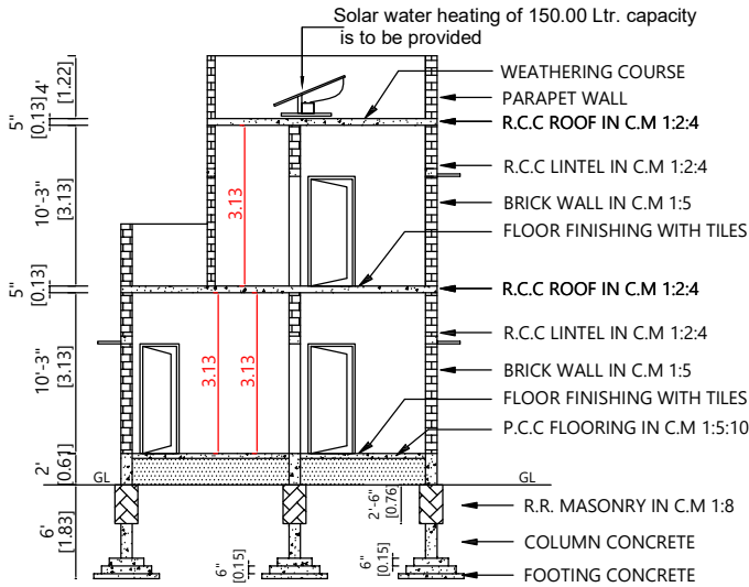
CROSS SECTION "AB"
