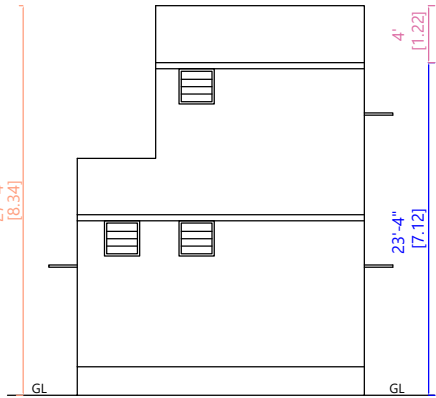
FRONT ELEVATION (WEST SIDE VIEW)
