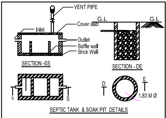
SEPTIC TANK & SOAK PIT DETAILS
