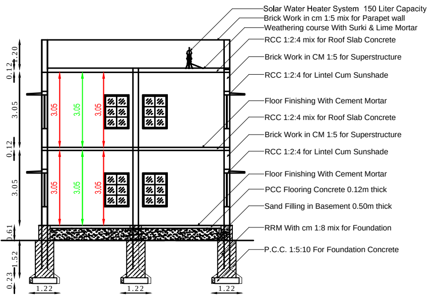
SECTION "AB"
