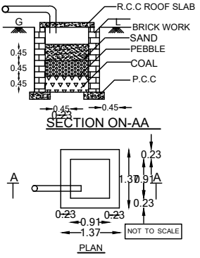
ORGANIC FILTRATION BED
