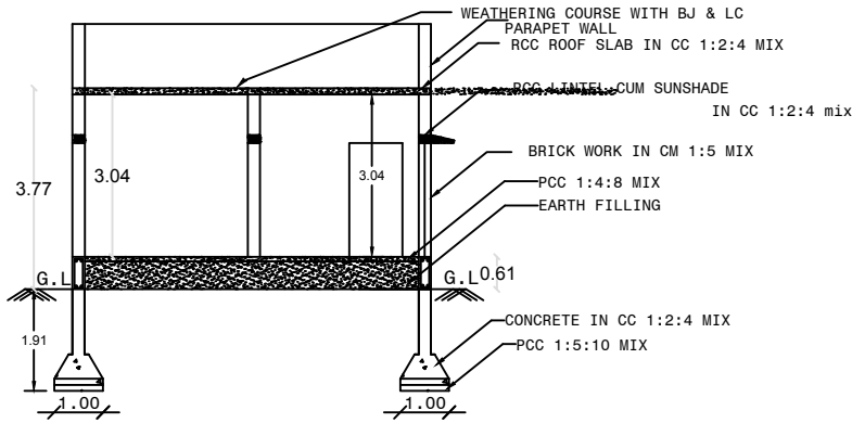
CROSS SECTION ON 'AA'
