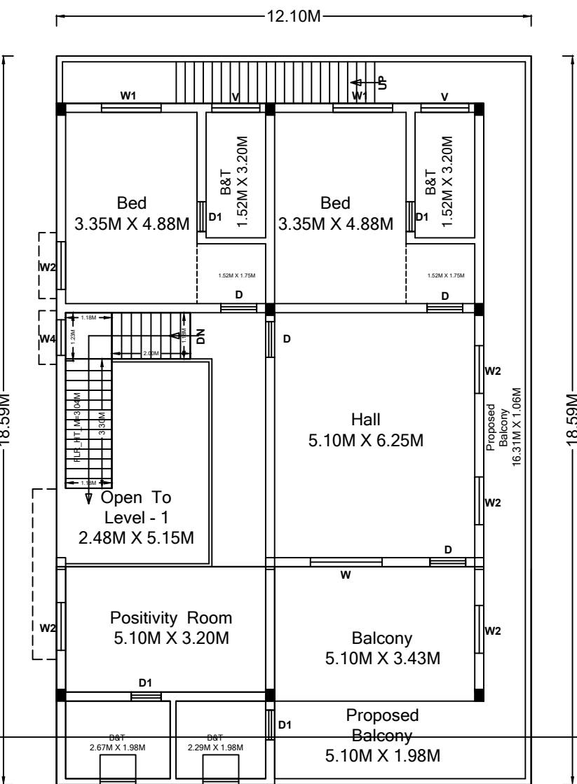
FIRST FLOOR PLAN SCALE : 1:100 (EXISTING, PROPOSED)
