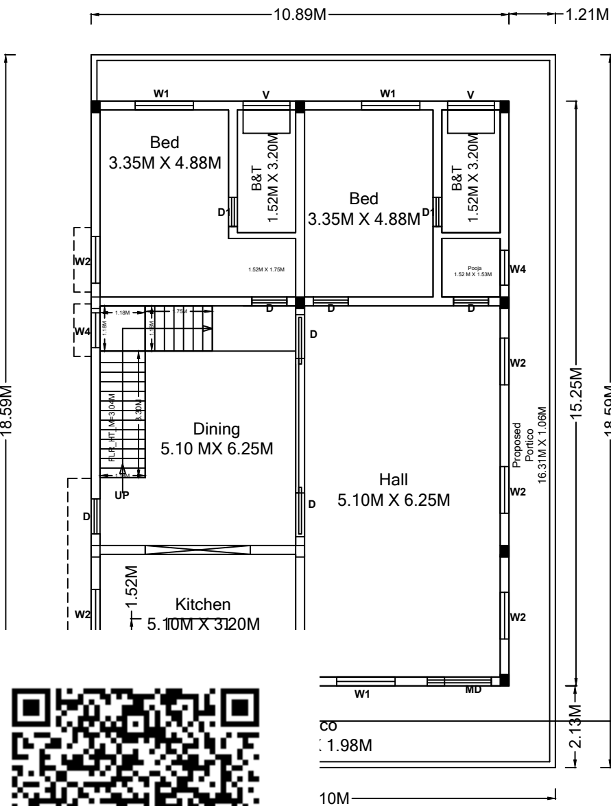
FLOOR PLAN SCALE : 1:100 (PROPOSED)
