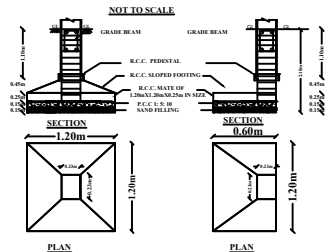
COLUMN FOOTING DETAILS
