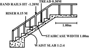
STAIRCASE DETAILS
