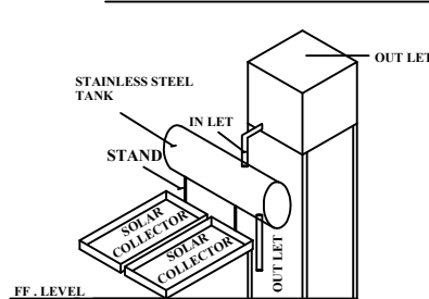
SOLAR HEATING WATER SYSTEM
