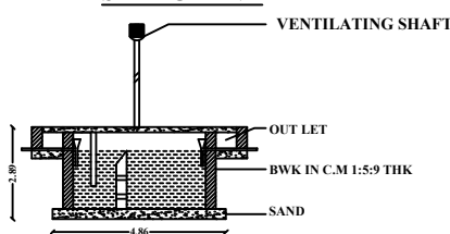
SEPTIC TANK
