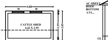
CATTLE SHED-PLAN
