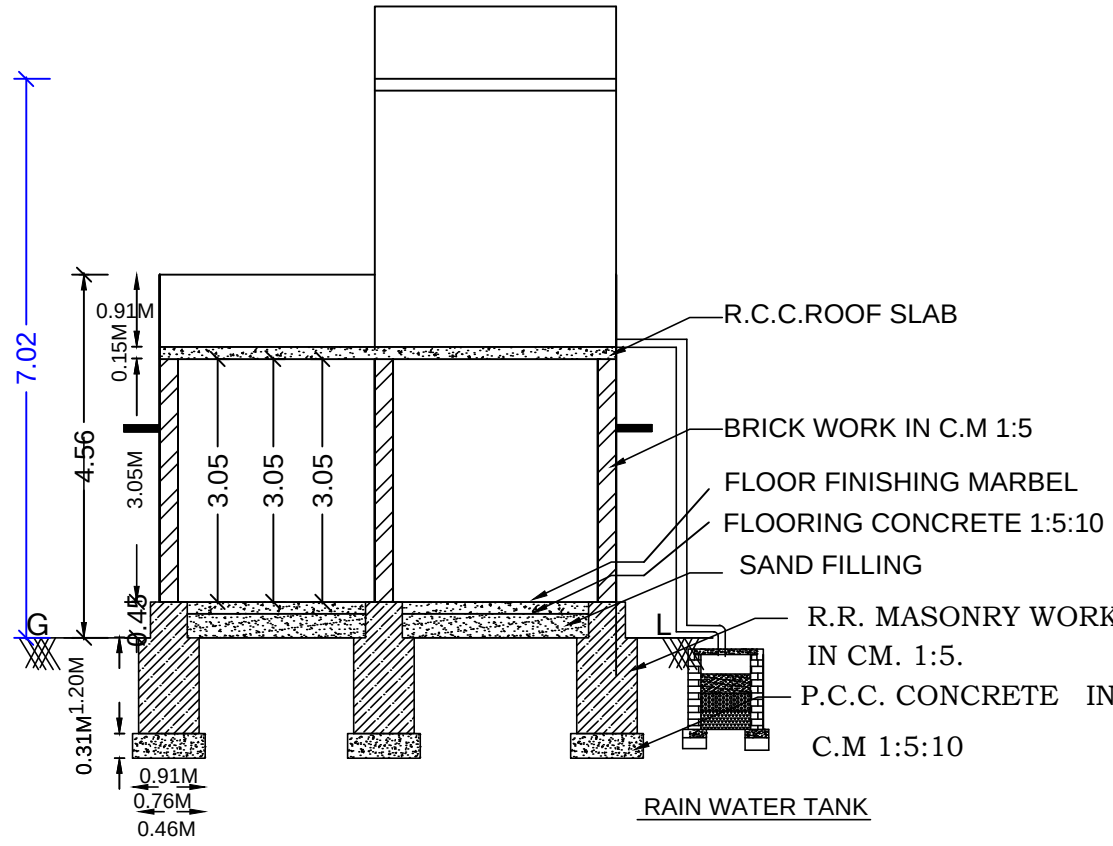
SECTION - XX
