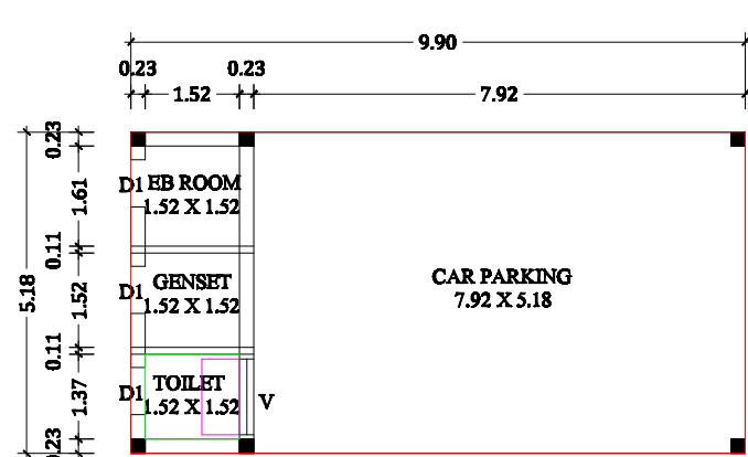
GROUND FLOOR PLAN BLOCK II
