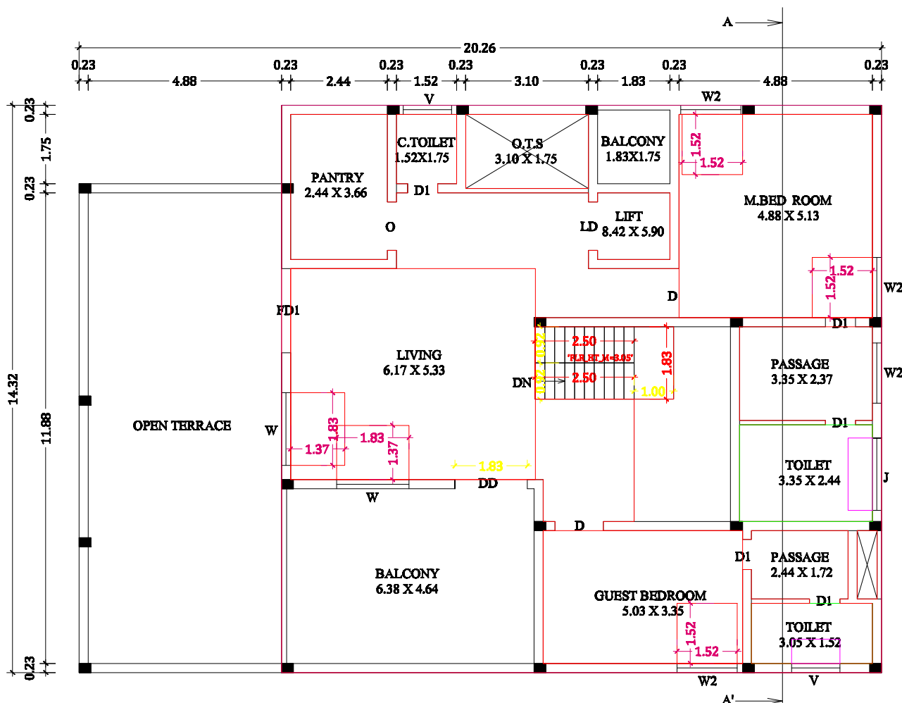
FIRST FLOOR PLAN BLOCK I
