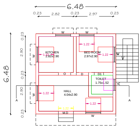
GROUND FLOOR BUILDING
