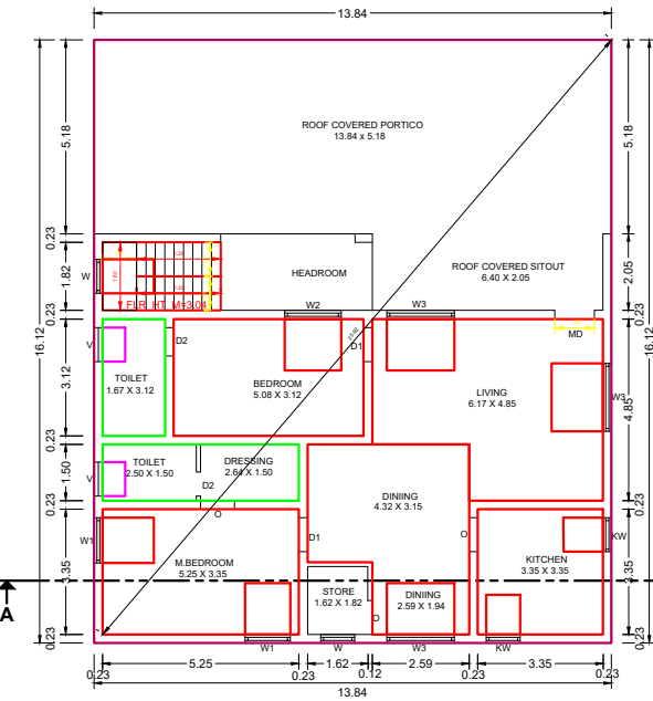
GROUND FLOOR PLAN (FLOOR-GROUND)
