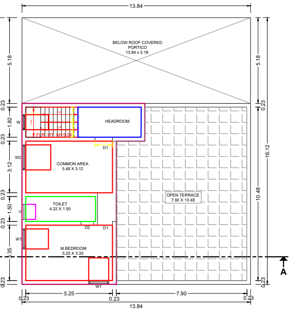
FIRST FLOOR PLAN (FLOOR-01)
