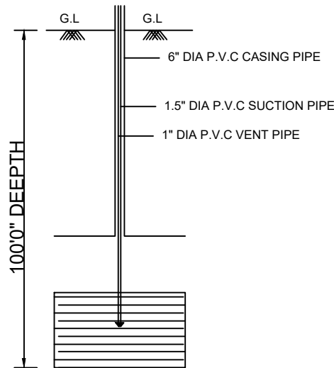
BORE WELL
