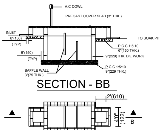
PLAN OF SEPTIC TANK
