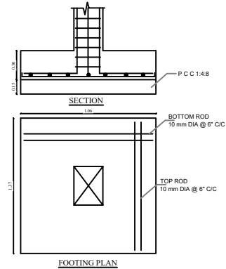
FOOTING PLAN
