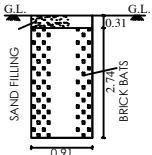
DETAILED PLAN OF RAINWATER PERCUSSION AND COLLECTION PIT
