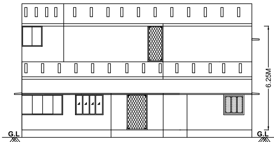
FRONT ELEVATION
