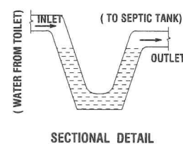
SECTIONAL DETAIL
