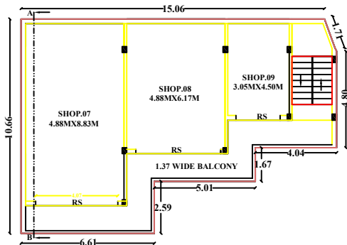
PROPOSED COMMERCIAL FIRST FLOOR - PLAN
