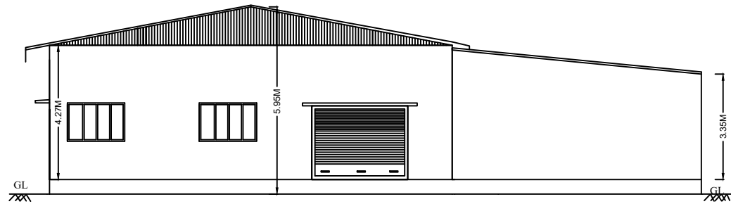
FRONT ELEVATION
