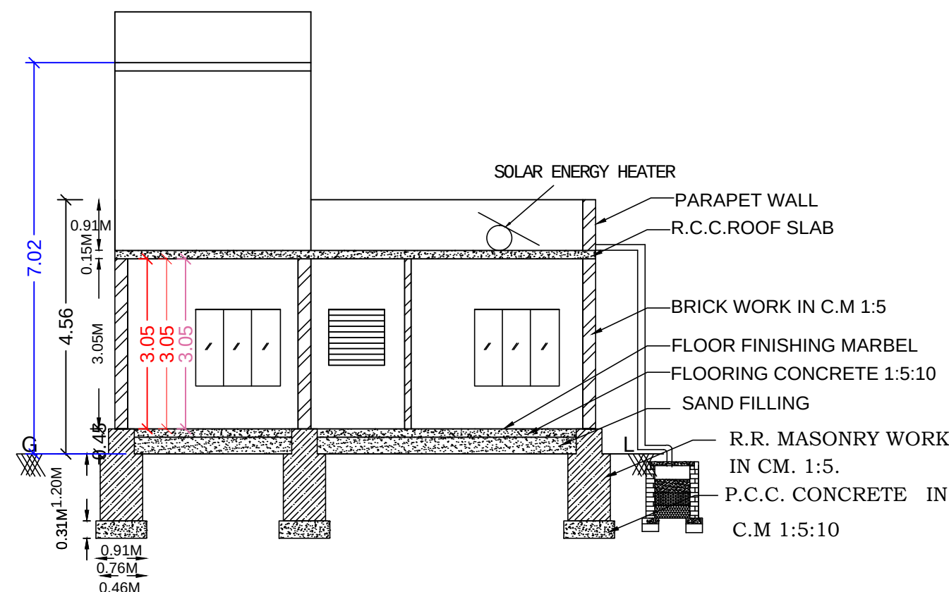
SECTION - XX
