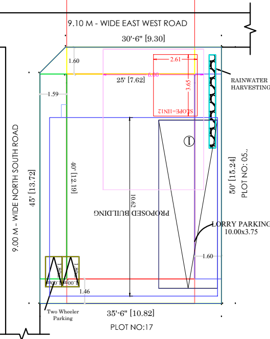
AREA OF THE PROPOSED CONSTRUCTION DETAILS
