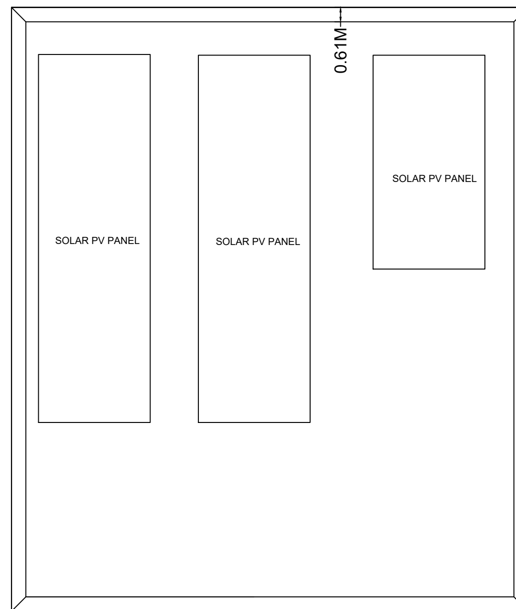
TERRACE ROOF AREA
