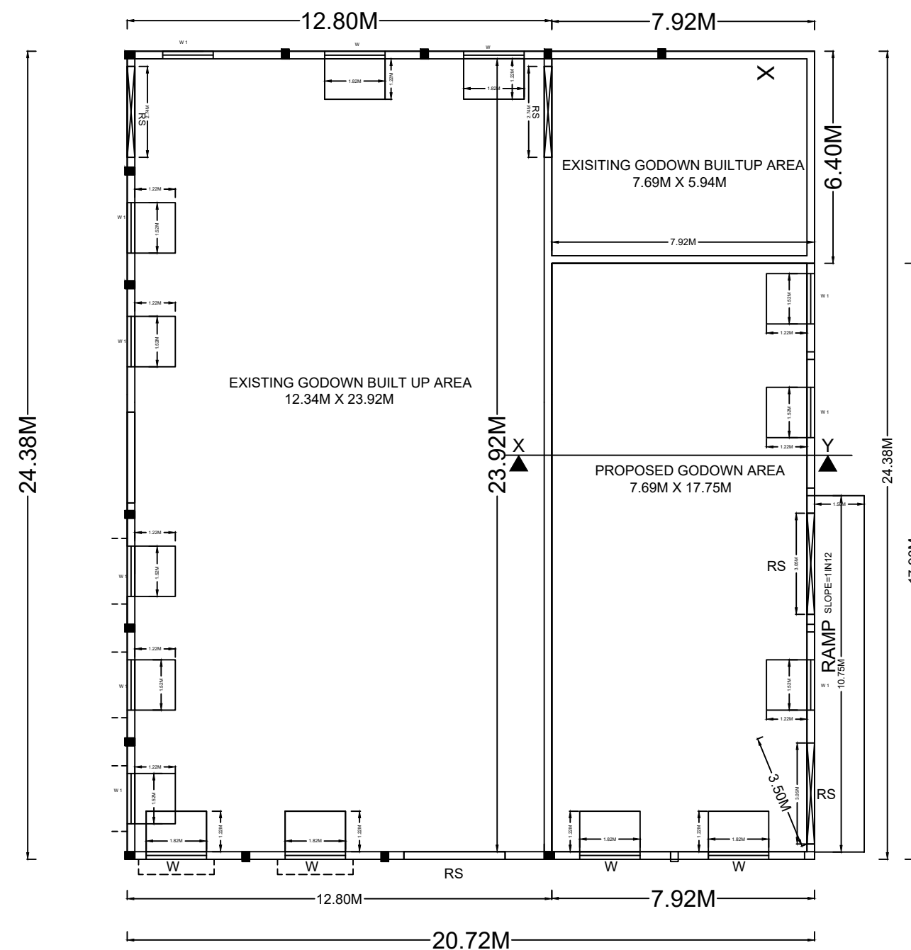
EXISTING & PROPOSED GROUND FLOOR PLAN
