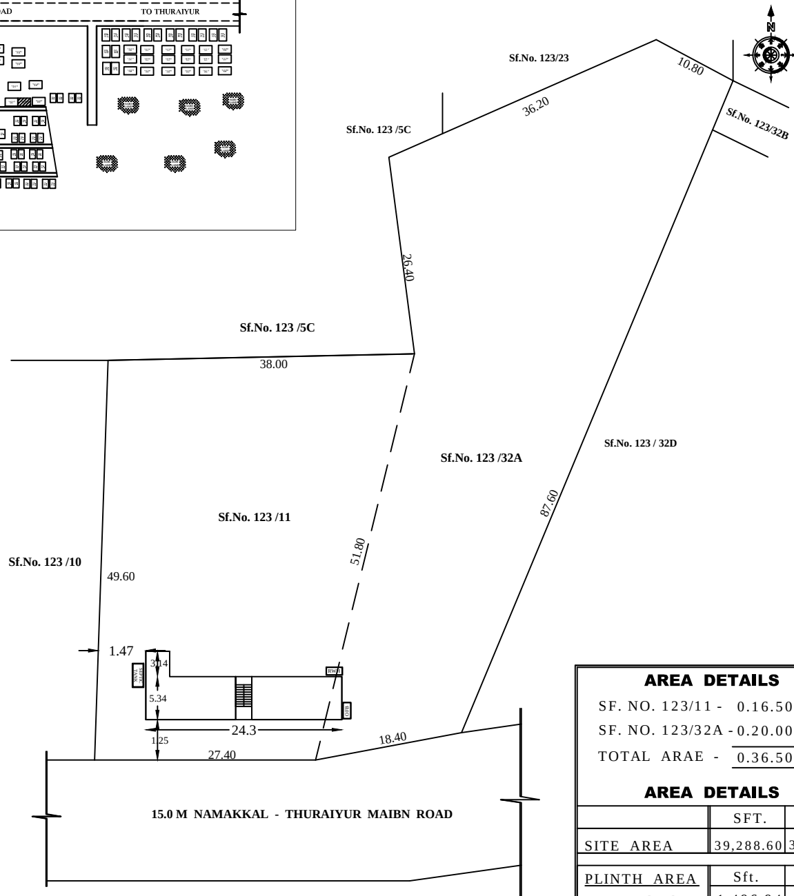
SITE PLAN (1:100)
