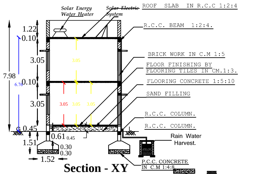
Section - XY
