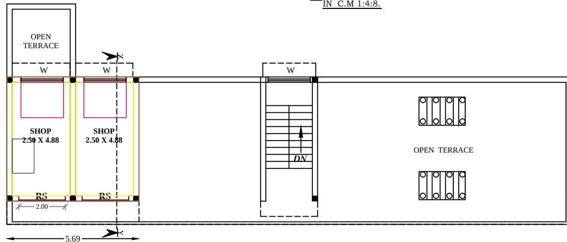
First Floor Plan. (Scale - 1:100)
