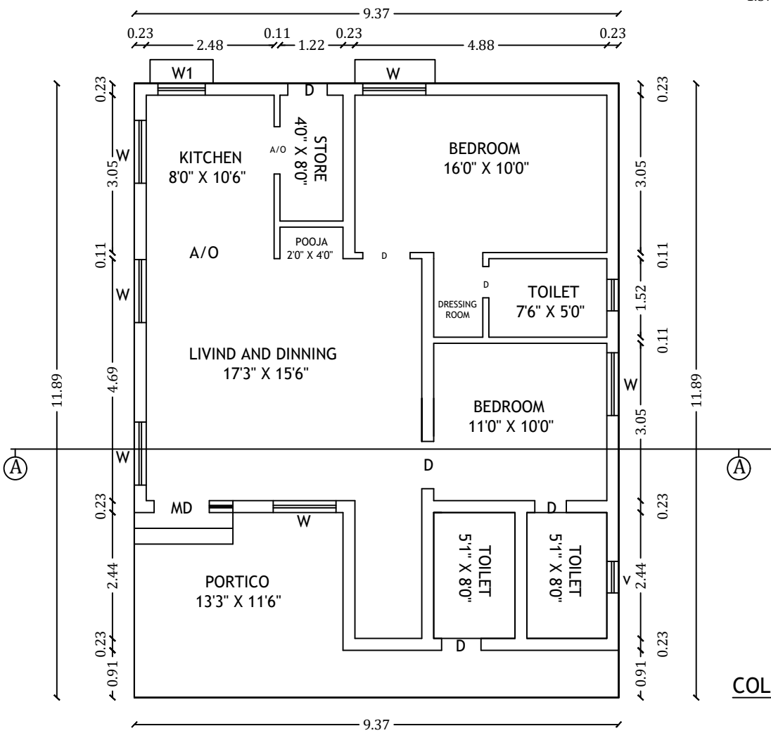
PLAN
