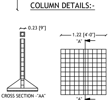
COLUMN DETAILS:-
