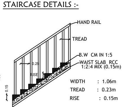
STAIRCASE DETAILS :-
