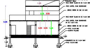
CROSS SECTION ON "AA"
