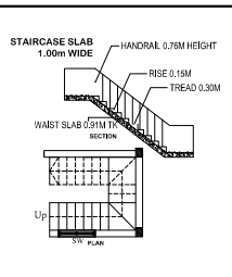
STAIRCASE SLAB 1.00m WIDE
