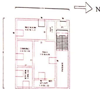
SITE PLAN SCALE = 1:100
