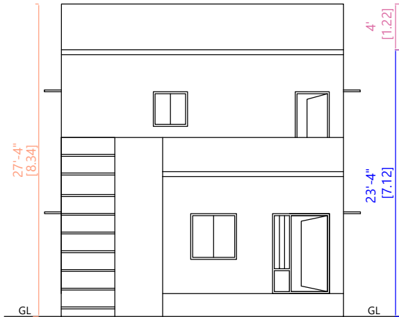
FRONT ELEVATION (EAST SIDE VIEW)
