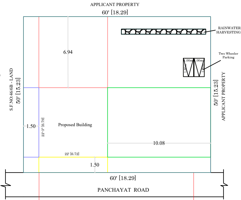
AREA OF THE PROPOSED CONSTRUCTION DETAILS
